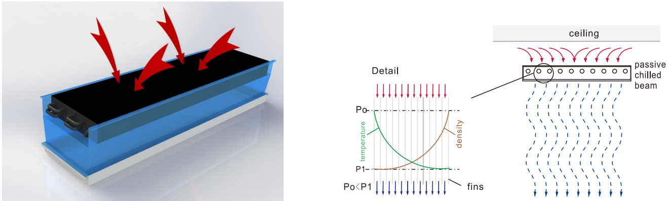
Figure 3: Passive Chilled Beam Natural Convection
